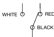
LEM7LSC SPDT CONTACT
