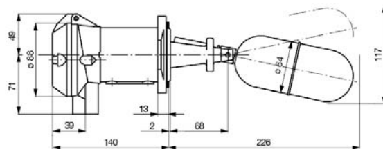
Flange dimension
