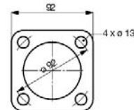
Flange dimension
