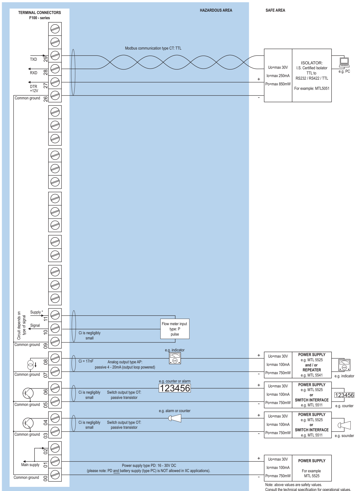
Configuration example IIB / IIC - F118-P-AP-CT-OT-PD-XI - Power requirement 16 - 30V DC
