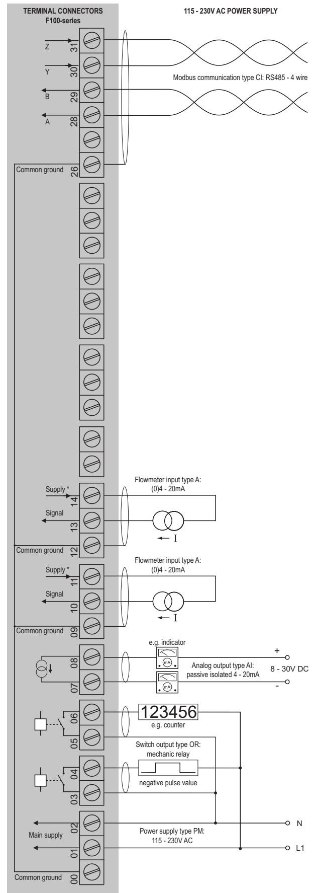
Configuration example F116-A-AI-CI-OR-PM-XX-ZX
