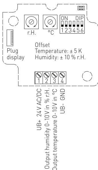
Schematic diagram AAVTF-U with display
