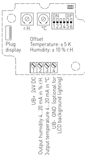
Schematic diagram AAVTF-I with display
