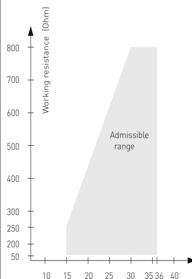
Load resistance diagram AAVTF-I 4...20 mA
